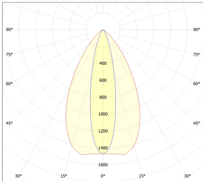
Polar Curve:
